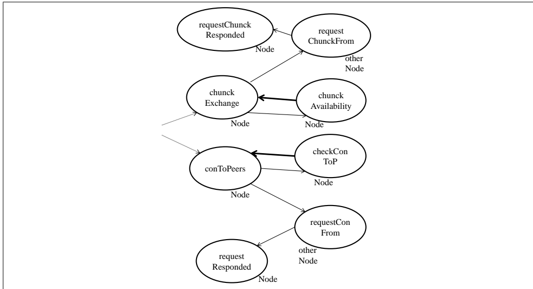
Figure 15: Event graph of connecting to the peers and downloading chunks from them.
