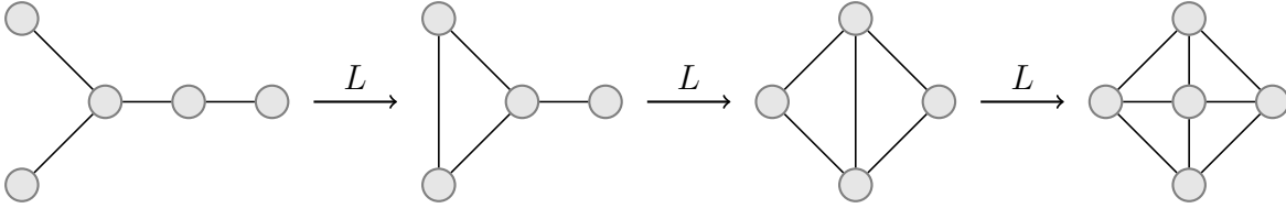
Figure 5: Iterating the line graph construction
