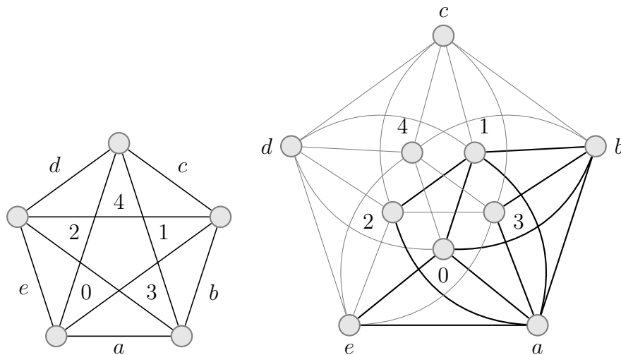
Figure 4: The clique K_5 and its line graph, where edges mentioned in the proof of Theorem 4 are drawn thicker
