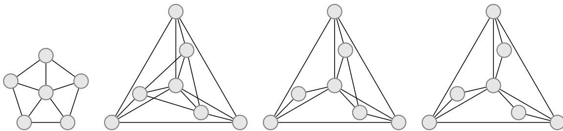
Figure 2: Minimal non-representable graphs
