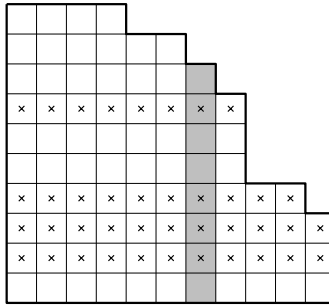
Figure 6: A Ferrers diagram with one \diamond -column, indicated in gray. The rows with crosses are the rightist rows of D .
