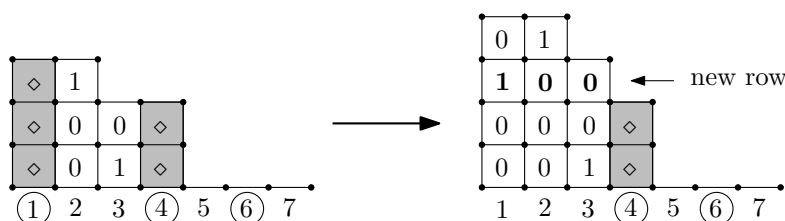
Figure 3: A substitution into the first column of a partial filling, involving an insertion of a new row between the second and third rows of the original partial filling.
