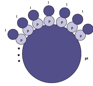
Figure 3: A family of interference graphs with unbounded price of anarchy.
