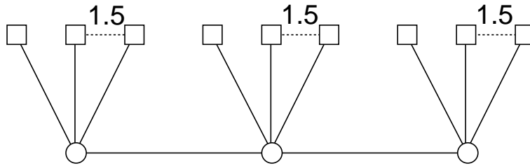
Figure 3: The graph Z_{1,3,0} .
