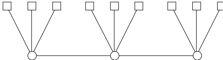
Figure 2: A short 3-rake
