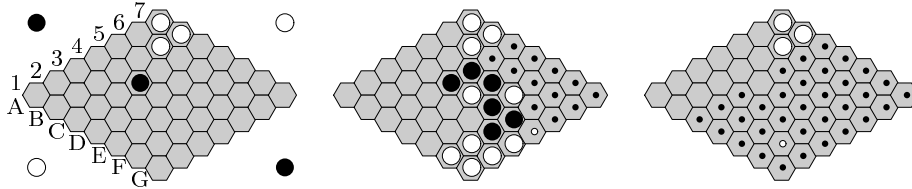
Fig. 8. SOLVER solves b6-c4. As shown by the SOLVER b6 recursion tree in Figure 13, c4 is the first black response considered to the white b6 opening (left). Following the topmost path b6-c4-f2-d5-d4-c5-e5-e4-g3-f3-g2-f4 in the recursion tree and applying Theorem 5 after f2 leads to the first solved state (center, with white win-weaklink); since f4 is a leaf of the recursion tree, the white win-weaklink here was discovered statically. SOLVER continues solving the c4-subtree, eventually determining that c4 is a black loss (right, with white win-weaklink). This win-weaklink does not contain c4 or b5, so, of the 13 possible b6-responses corresponding to the initial black mustplay region described in Figure 7, 11 moves remain to be checked.
