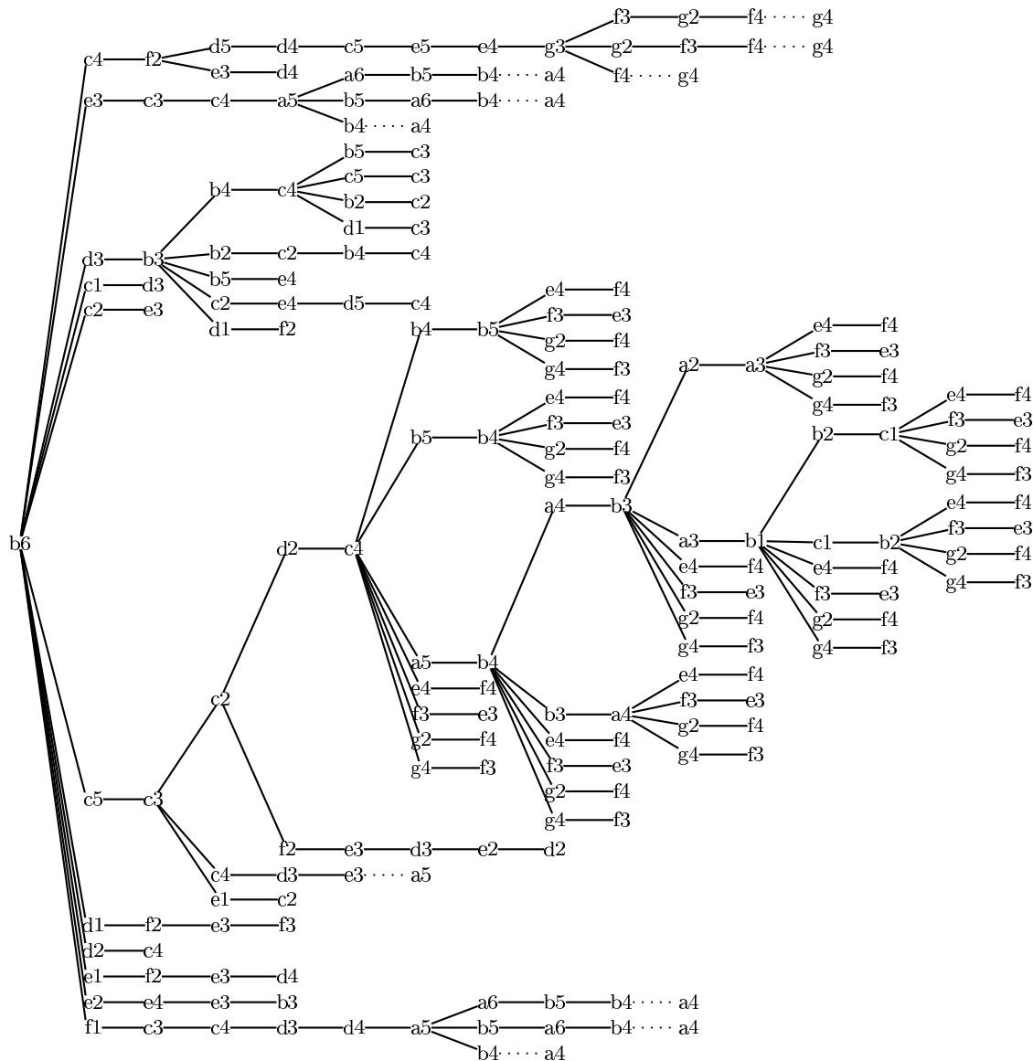
Fig. 13. The SOLVER recursion tree for the 7 \times 7 opening White-b6 (with the ten nodes connected by dotted edges added so that every path ends with a winning move). For each node, the order of child generation is top-to-bottom. Each SOLVER recursion tree is a subtree of the complete game-tree, as the only replies to a winning move which appear in the recursion tree are those replies in that state's mustplay region. For example, consider for the tree shown here the state G after White plays b6. As shown in the last diagram in Figure 8, White has a win-weaklink created by playing at c4 which does not contain b5; thus b5 is not in the Black mustplay region for G , so SOLVER never needs to consider the Black move to b5, so b5 does not appear as a child of b6 in this recursion tree. Notice from the tree shown here that in solving the b6 opening the selection of d2 as the first move considered at the b6-c5-c3-c2 subtree was unfortunate, as d2 leads to a White loss whereas f2, the second move considered, leads to a White win. If f2 had been considered first, the d2 subtree would not have been explored, and the resulting recursion tree would have had only 97 nodes instead of 197.
