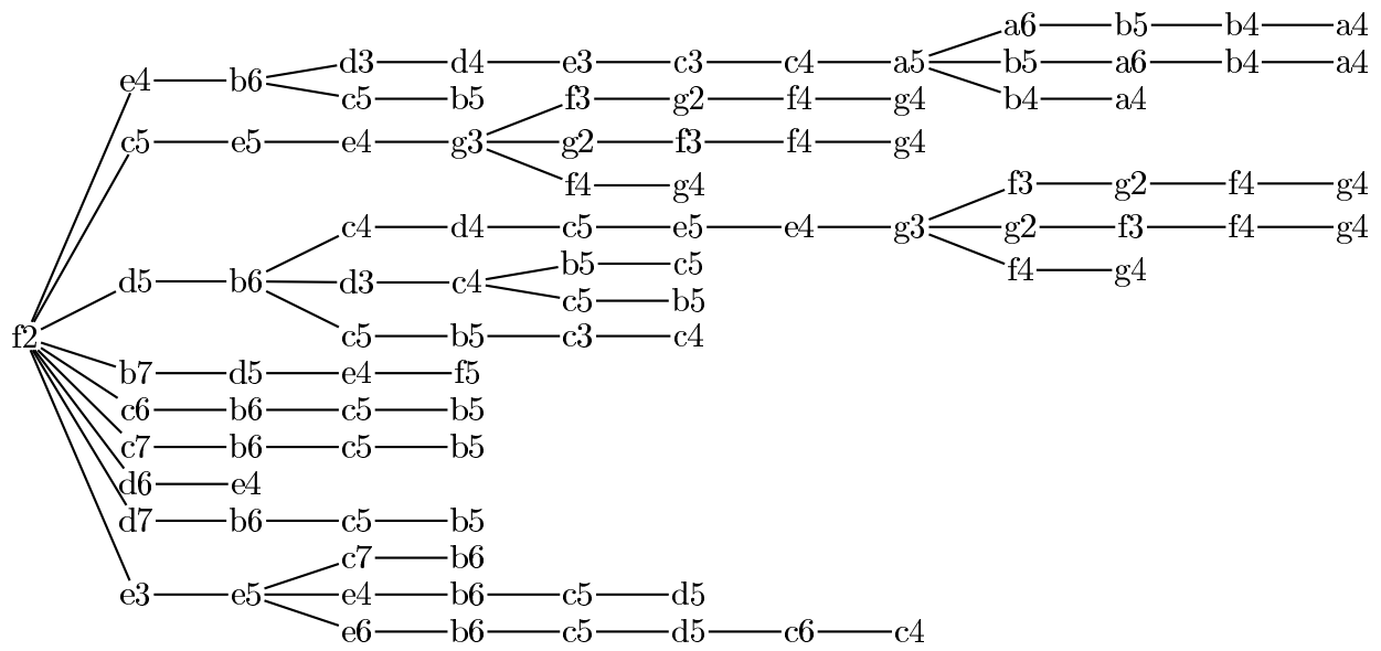
Fig. 16. A SOLVER proof tree for the 7x7 opening White-f2. The data for this tree was generated by first running a modified version of SOLVER in which the final move considered from any position is a winning move; this guarantees that every recursion tree path ends with a winning move. The resulting recursion tree was then pruned, at all points in the tree, by removing any losing moves made by the winning player before the winning move for that state was found.
